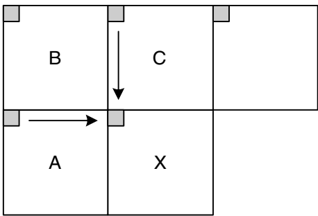
Figure 5.14 Prediction of DC coefficients
