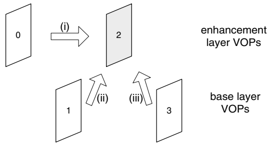
Figure 5.62 Temporal enhancement P-VOP prediction options
