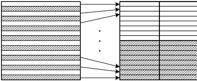
Figure 5.25 Field DCT
