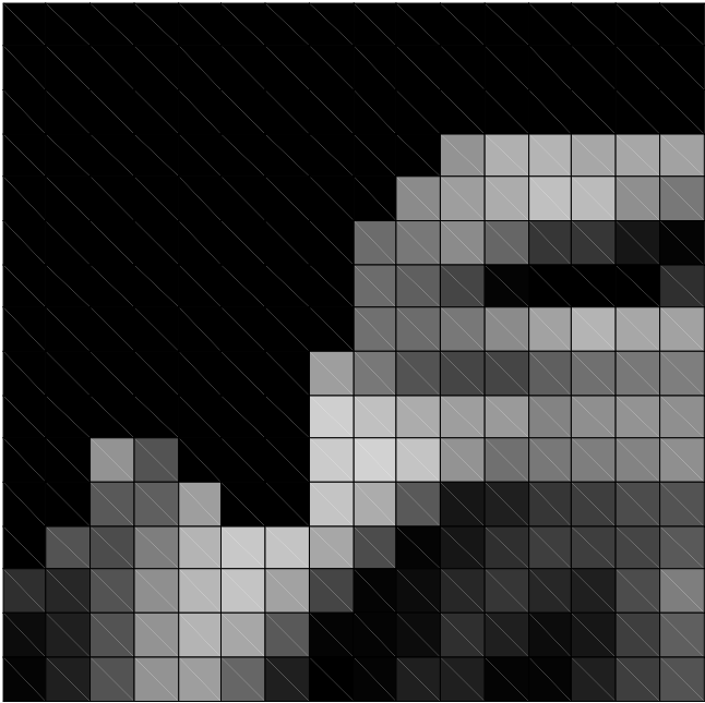
Figure 5.38 Boundary MB
