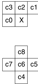
Figure 5.35 Context template for inter BAB
