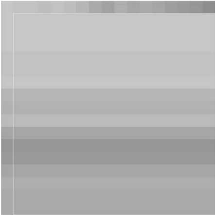
1 (horizontal), SAE = 5097
