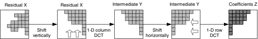
Figure 5.55 Shape-adaptive DCT
