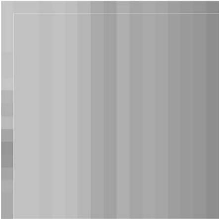
0 (vertical), SAE = 3985
