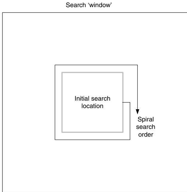
Figure 7.7 Full search (spiral scan)
