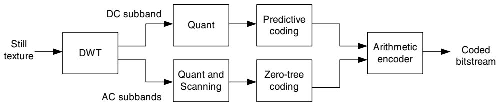
Figure 5.68 Wavelet still texture encoder block diagram
