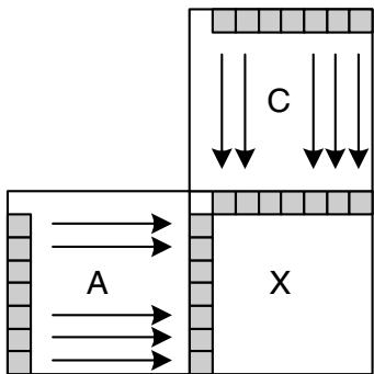
Figure 5.15 Prediction of AC coefficients
