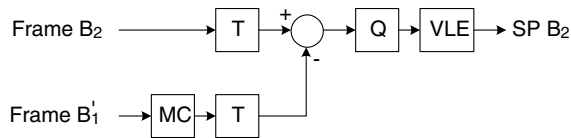
Figure 6.51 Encoding SP-slice B_2 (simplified)
