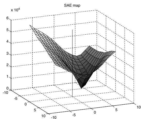
Figure 7.5 SAE map
