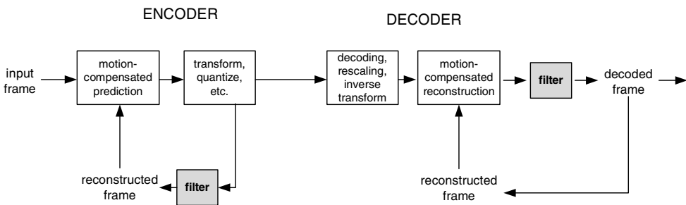
Figure 7.22 Loop filter implementation
